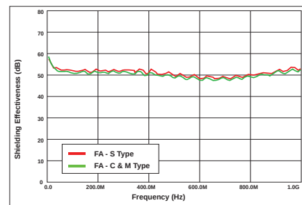
Typical SE in S, C, & M Type Construction
