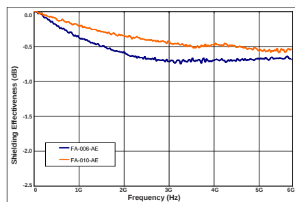
Typical Absorption in A Type Construction
